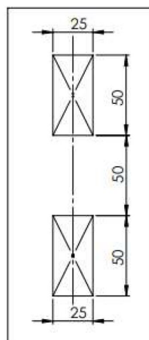
PANEL CUTOUT
